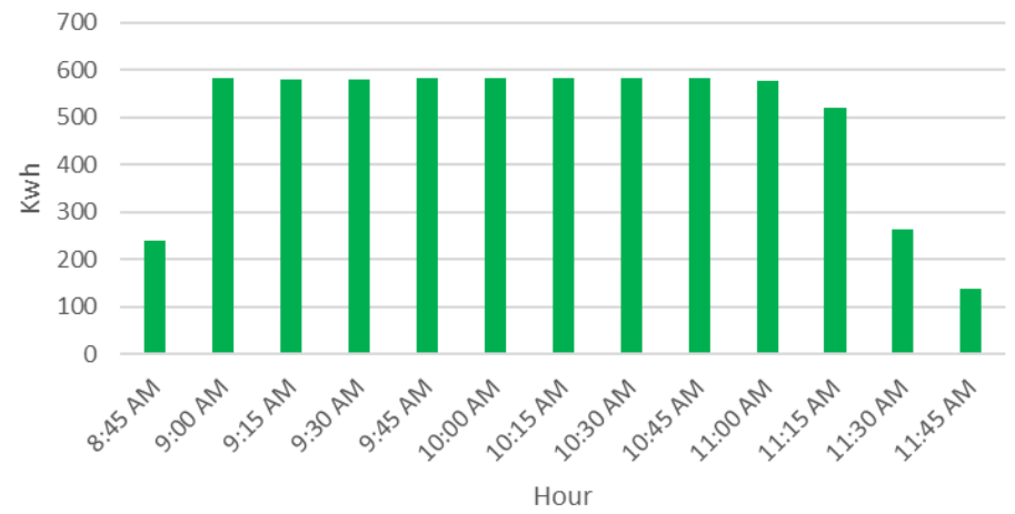
Kwh Charge on Nov. 4, 2018
