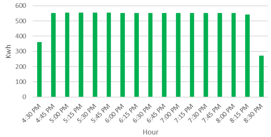
Kwh Charge on Apr. 29, 2018
