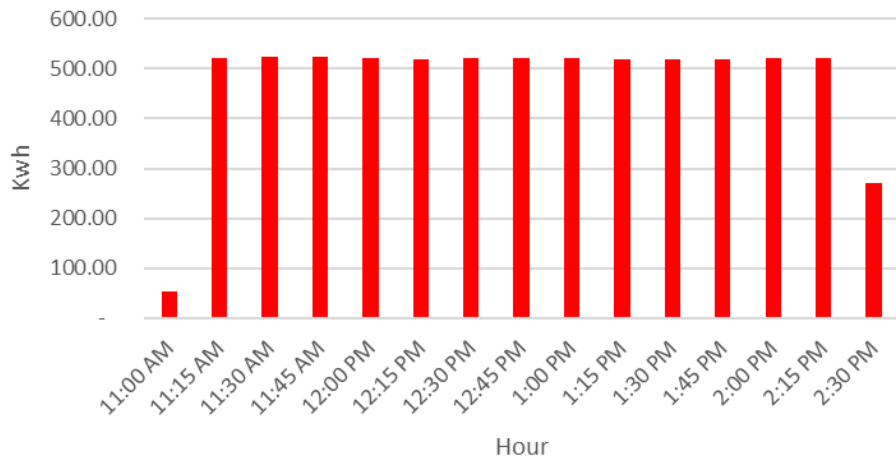
Kwh Discharge on Mar. 31, 2018
