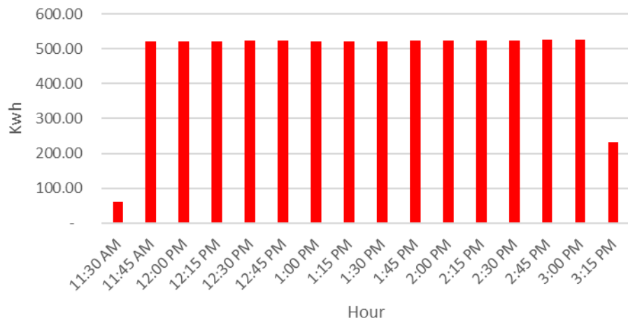
Kwh Discharge on Mar. 3, 2018
