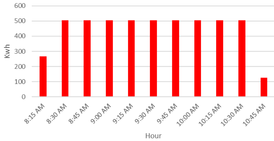
Kwh Discharge on Jan. 7, 2018
